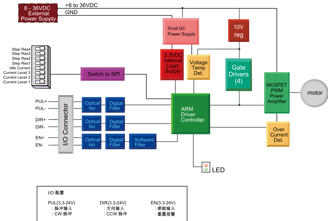
DM422 Block Diagram
